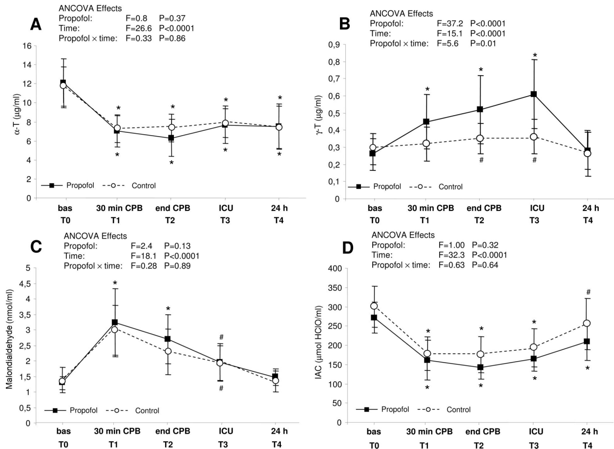
Fig. 2. Time course of \alpha -tocopherol ( \alpha -T; A ), \gamma -tocopherol ( \gamma -T; B ), malondialdehyde ( C ), and individual antioxidant capacity (IAC; D ) plasma levels, during and after surgery. Blood was collected before induction of anesthesia (bas, T 0 ), 30 min after the beginning of cardiopulmonary bypass (30 min CPB, T 1 ), after protamine administration and on-pump weaning (end CPB, T 2 ), at arrival in the intensive care unit (ICU, T 3 ), and 24 h after anesthesia induction (24 h, T 4 ). Data are mean and SD. * P < 0.001 and # P < 0.05 versus baseline, after controlling for multiple testing. Data were analyzed as delta values versus baseline and compared between the two anesthesia regimens by repeated-measures analysis of covariance (ANCOVA) with a group \times time factorial design.
